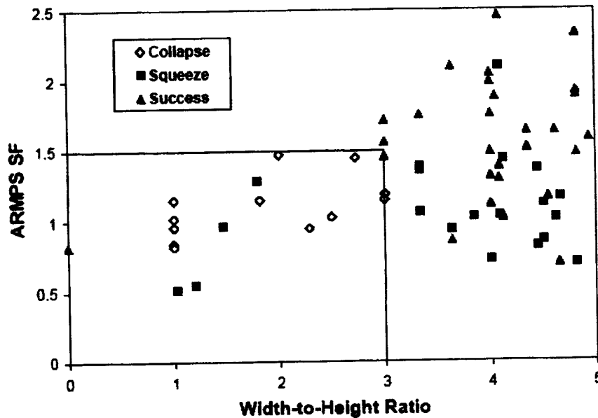
Figure 2. NIOSH's Database for Sudden Massive Collapse (from Mark 2006)
