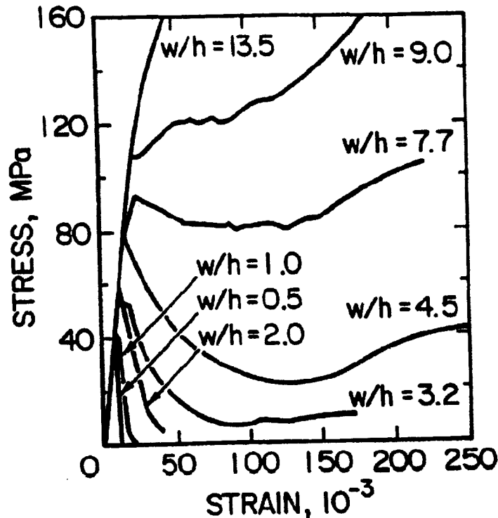
Figure 1. Effect of Pillar to Height Ratio on the Behavior of Coal Pillar (from Mark 2006)
